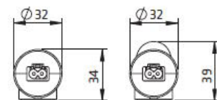
Dimensions for screw mounted On / Off switch
