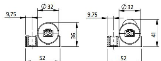
Dimensions for screw mounted On / Off switch
