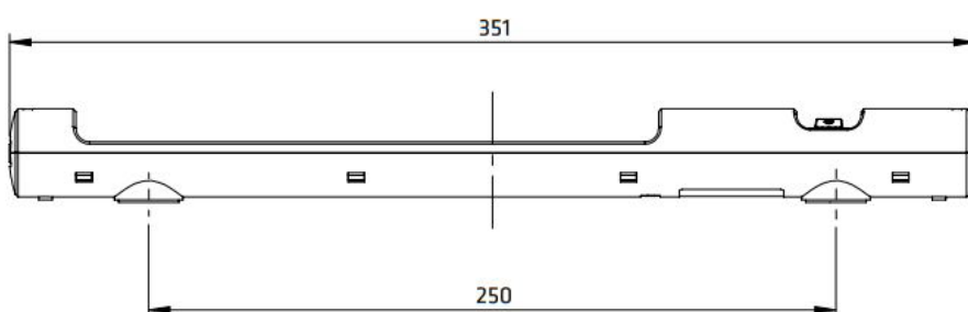
Dimensions for magnetic / screw mounted
